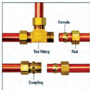
Fig. 5.28: Compression joints
