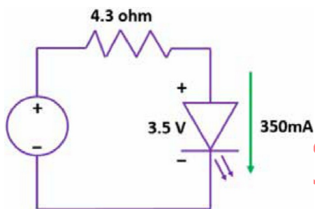
Fig. 5.9: Working of LED drivers
