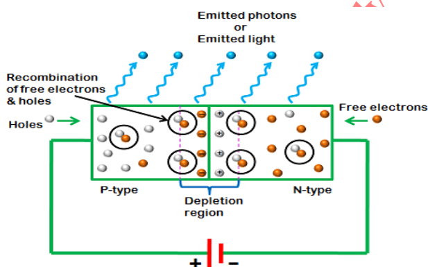
Fig. 5.4: Working of LED
