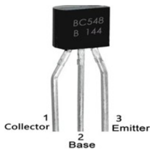
Fig. 3.14 Transistor image
