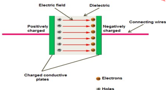
Fig. 3.8: Construction of Capacitor
