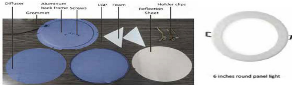
Fig 6.28: Round Panel light parts
