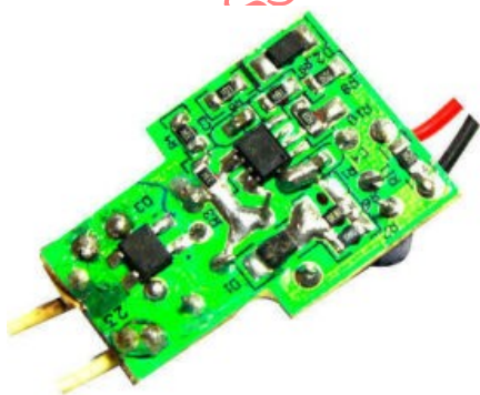
Fig. 6.13: LED driver in Housing
