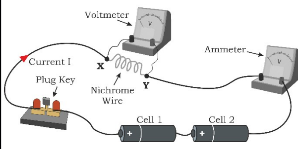
Fig. 2.34: Circuit diagram of Ohm's Law
