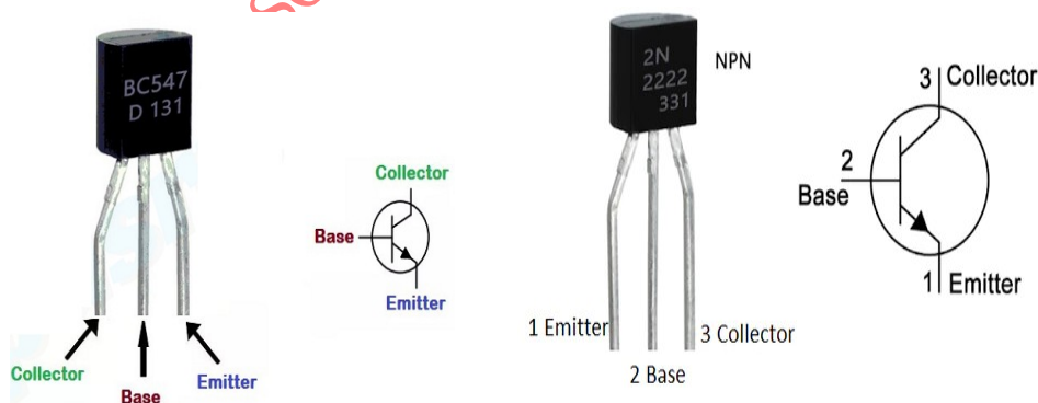
Fig. 3.16: NPN transistors-BC547 and 2N2222
