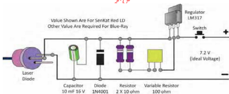
Fig. 7.3: Components of a Typical LED Driver
