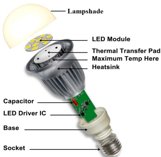
Fig. 6.10: LED Lamp
