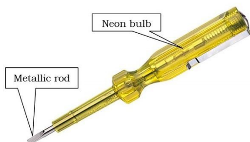
Fig. 4.5: Phase Tester
