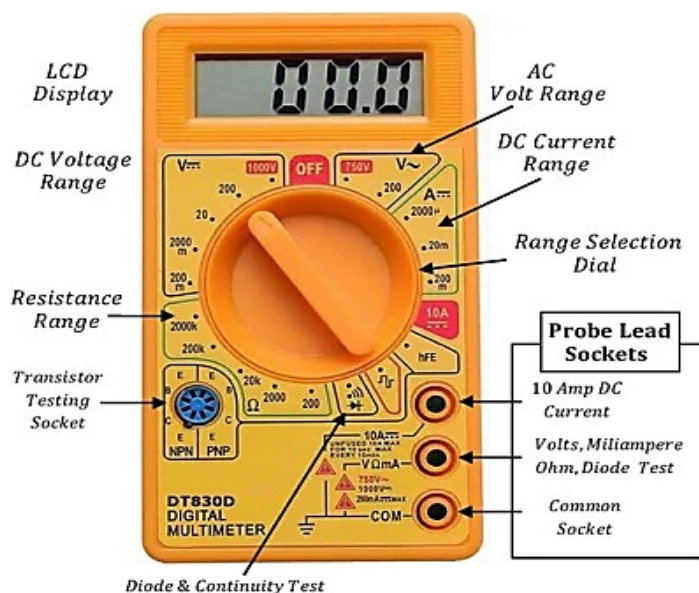
Fig. 4.11: Measurements Using Multimeter
