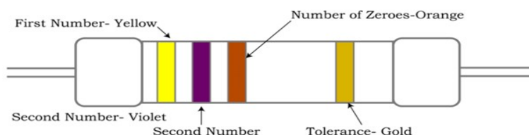
Fig. 3.4: Four band Resistor Specification
