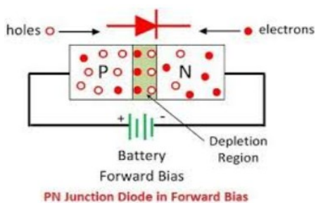
Fig. 3.11: P-N Junction Diode working in forward bias
