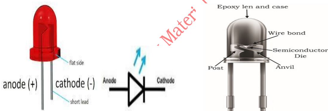
Fig 3.13: (a) Light emitted diode (LED) (b) symbol of LED (c) Internal parts of LED
