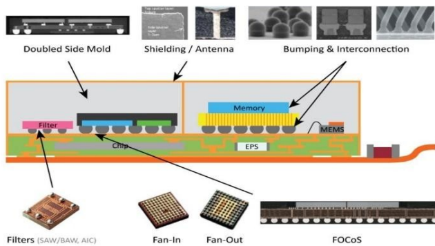
Fig. 1.19: Advanced IC Packaging
