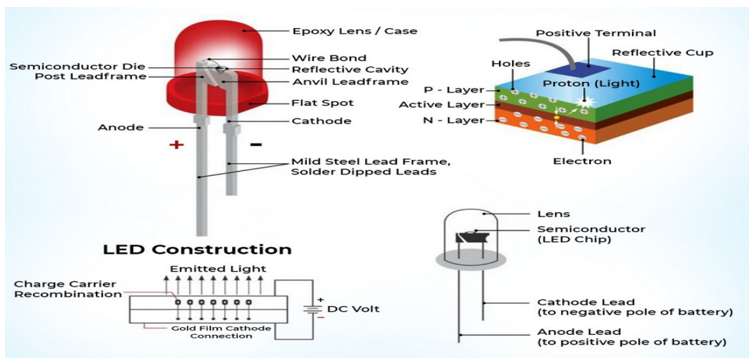
Fig. 5.3: Construction of LED
