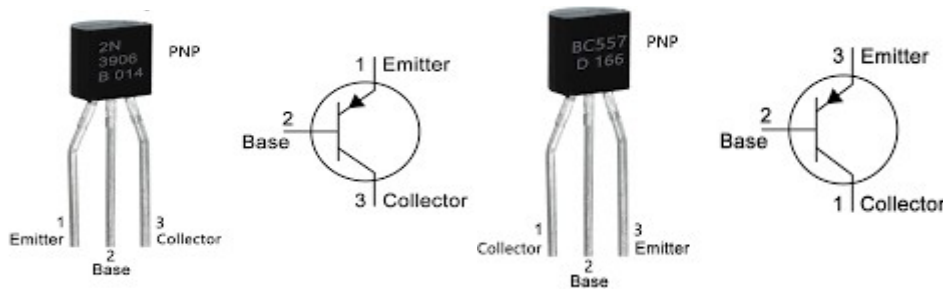
Fig. 3.17: PNP transistors-2N3906, BC557
