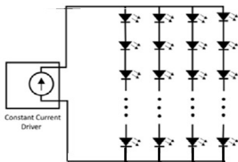
Fig. 5.11: Parallel Connection
