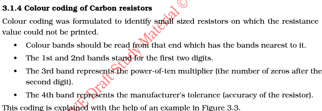
RESISTOR COLOUR CODES
