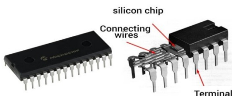
Fig. 3.19 Integrated Circuit
