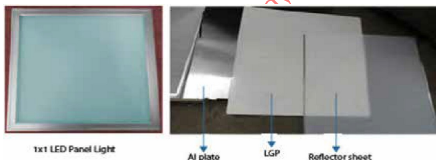
Fig. 6.30: 1x1 and 2x2 Square Panel Light
